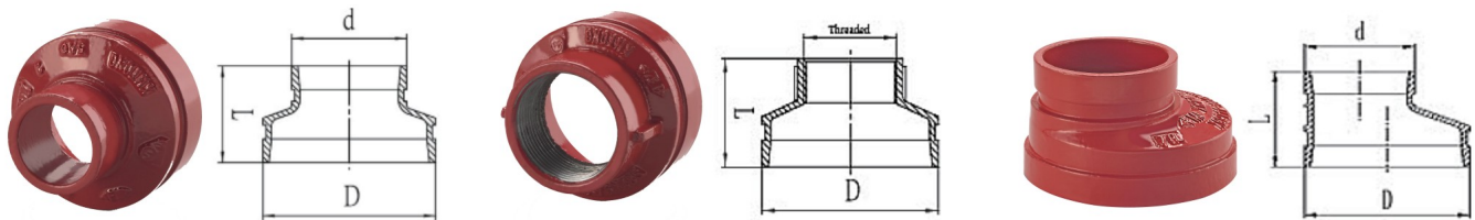
GROOVED / THREADED CONCENTRIC REDUCER 정심레듀샤 - 07/ 07S
